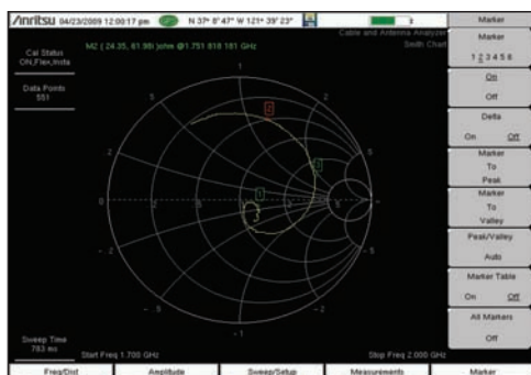
Smith Chart
